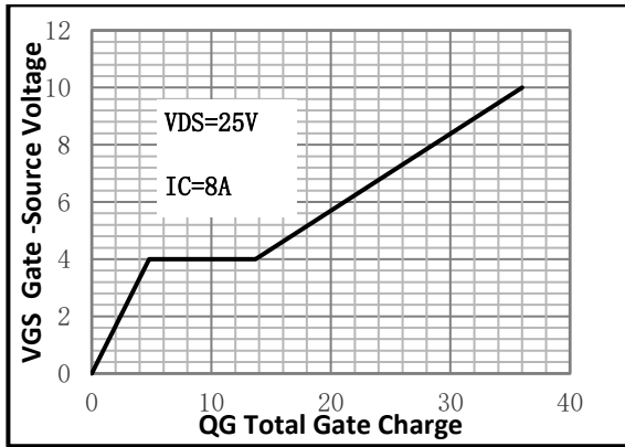
Fig.1 Gate-Charge Characteristics
