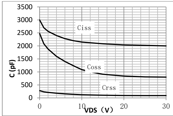
Fig.2 Capacitance Characteristics
